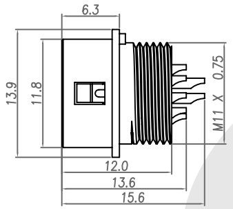
HOUSING + CONTACT + SHELL A
