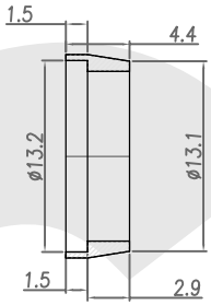
SHELL B
