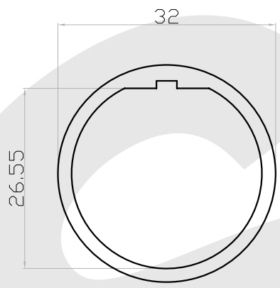
O-RING
