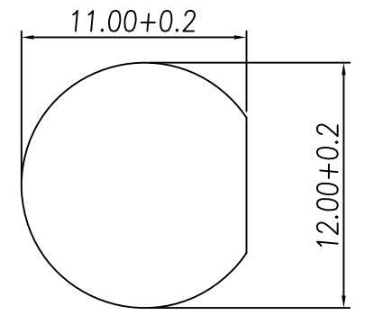
PANEL CUT-OUT
